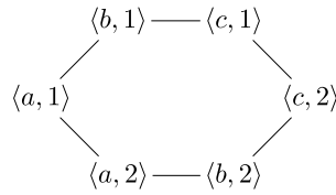
Fig. 1. Hasse diagram of pre-order \leq_p between profiles of \mathbb{P}_{\mathbb{L}} . A link between two profiles represents that the profile on the left precedes the one in the right. The reflexivity and transitivity of the pre-order is graphically omitted.
