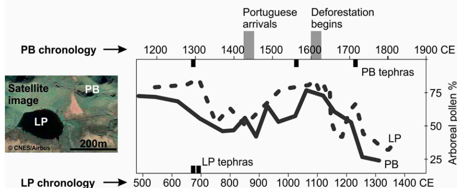
Fig. 1. Arboreal pollen trends and tephra layers at Lagoa do Peixinho (LP, ref. 1) and Pico Bog (PB, ref. 3) showing the mismatch between chronologies based on pollen concentrates (LP) and macrofossils/bulk dates (PB).
