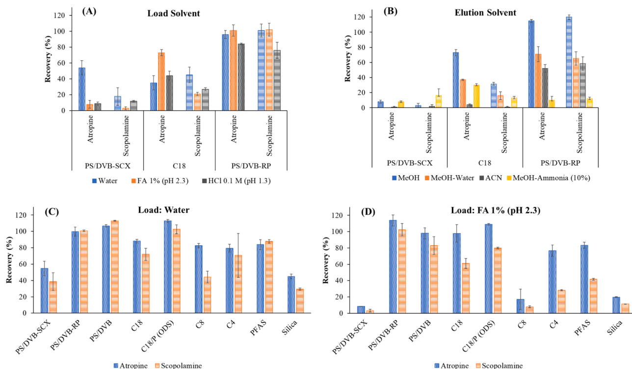
Fig. 2. Optimization of (A) sample loading solvent and (B) elution solvent and selection of the best sorbent after sample loading with (C) water and (D) formic acid (FA) 1%. See details of the full experimental conditions in section 3.1.1.
