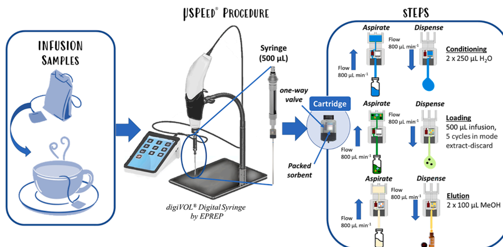
Fig. 1. Schematic diagram of the optimized \mu\text{SPEed}^{\text{®}} procedure using the digiVOL ® Digital Syringe (EPREP, Australia).
