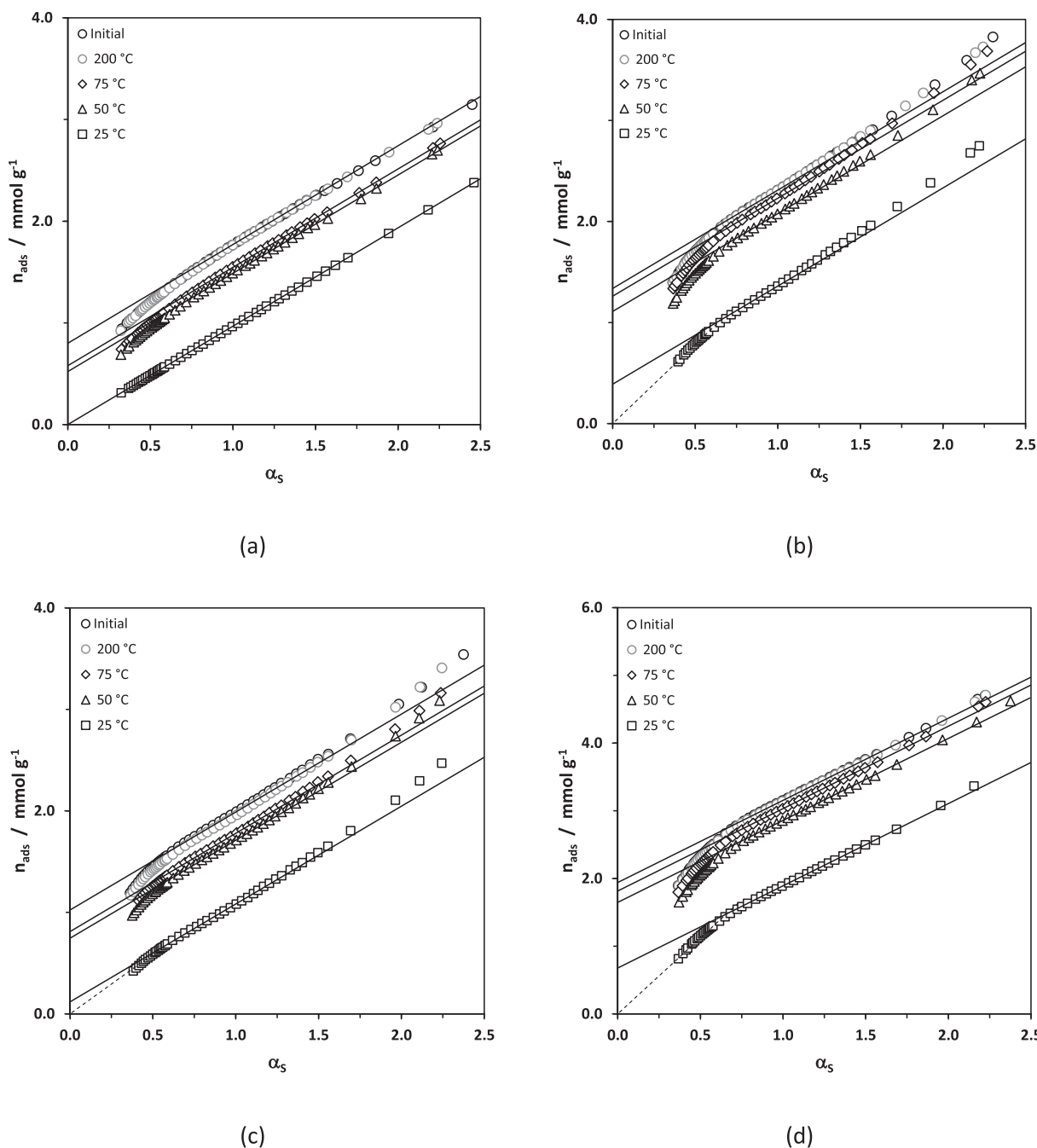
Fig. 3. \alpha_s plots corresponding to the nitrogen adsorption isotherms, at -196\text{ }^\circ\text{C} , determined on (a) Na-SD, (b) SD125, (c) Al-SD and (d) SD195, before (initial) and after n-nonane pre-adsorption with subsequent outgassing at increasing temperatures up to 200\text{ }^\circ\text{C} . (The amounts adsorbed are, in all cases, expressed per g of the corresponding initial material outgassed at 200\text{ }^\circ\text{C} ).
