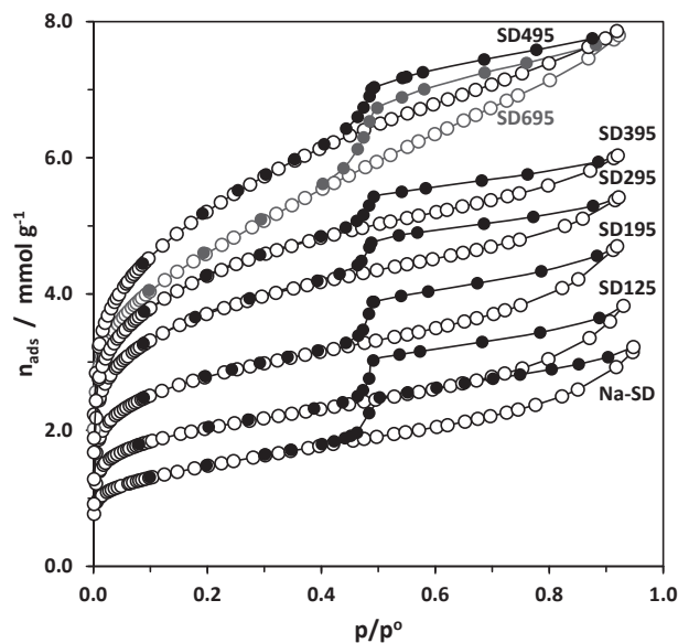
Fig. 1. Nitrogen adsorption-desorption isotherms, at -196\text{ }^{\circ}\text{C} , determined on Na-SD and acid treated with 1 M HCl at 25\text{ }^{\circ}\text{C} (120 min) and with 1, 2, 3, 4 and 6 M HCl at 95\text{ }^{\circ}\text{C} (30 min).
