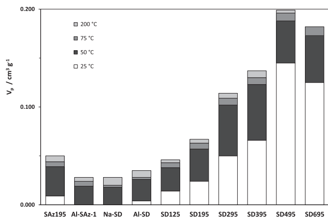
Fig. 6. Pore volumes, from which n-nonane is removed upon outgassing at increasing temperatures, obtained from the \alpha_S plots corresponding to nitrogen adsorption, at -196 °C, on Na-SD and ion-exchanged and acid treated Na-SD and SAz-1. (The pore volumes are, in all cases, expressed per g of the corresponding initial material outgassed at 200 °C).
