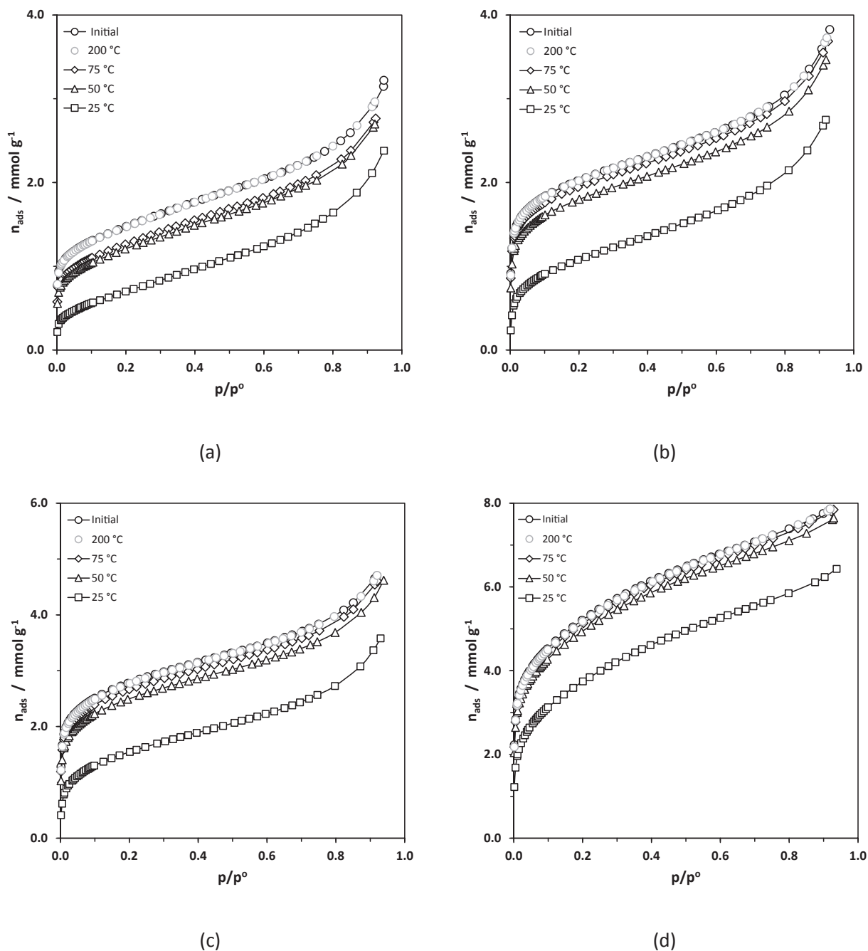
Fig. 2. Nitrogen adsorption isotherms, at -196\text{ }^{\circ}\text{C} , determined on (a) Na-SD, (b) SD125, (c) SD195 and (d) SD495, before (initial) and after n-nonane pre-adsorption with subsequent outgassing at increasing temperatures. (The amounts adsorbed are, in all cases, expressed per g of the corresponding initial material outgassed at 200\text{ }^{\circ}\text{C} ).
