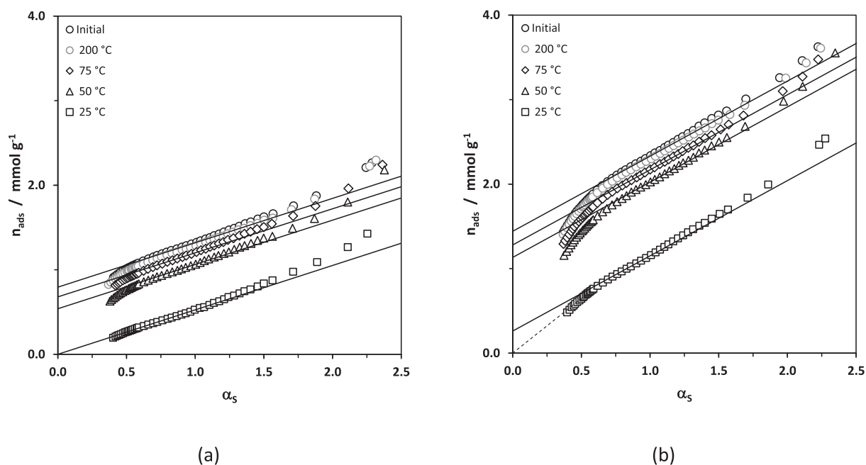
Fig. 5. \alpha_S plots corresponding to the nitrogen adsorption isotherms, at -196 °C, determined on (a) Al-Saz-1 and (b) SAz195 before (initial) and after adsorption of n-nonane with subsequent outgassing at increasing temperatures. (The amounts adsorbed are, in all cases, expressed per g of the corresponding initial material outgassed at 200 °C).
