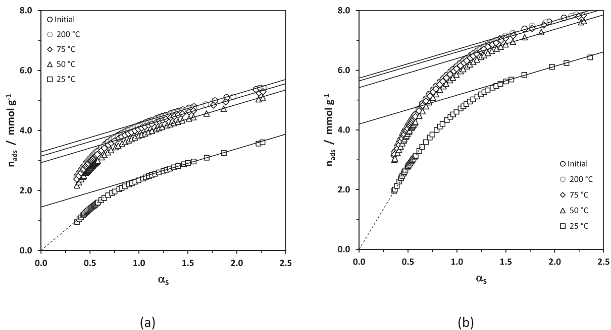
Fig. 4. \alpha_S plots corresponding to the nitrogen adsorption isotherms, at -196 °C, determined on (a) SD295 and (b) SD495, before (initial) and after n-nonane pre-adsorption with subsequent outgassing at increasing temperatures up to 200 °C. (The amounts adsorbed are, in all cases, expressed per g of the corresponding initial material outgassed at 200 °C).
